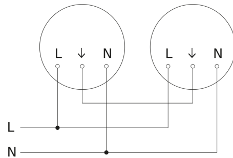
Master/master interconnection circuit diagram
